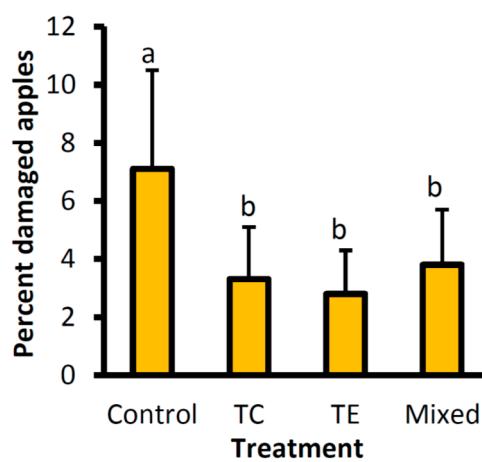
Figure 2. Average percent apples damaged by C. pomonella (±SE) in a completely randomized block experiment with four treatments; mass release using Trichocards® of T. evanescens (Te), T. cacoeciae (Tc), a mix of the two species (Mixed) and a control for years 2012 and 2013.
