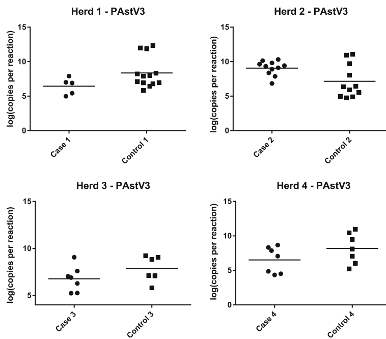
Fig. 2 Viral load (log 10 copies per reaction) of PASTV3. The copy number for the positive PASTV3 samples in herd 1–4 for case and control pigs. The straight line shows the mean value
