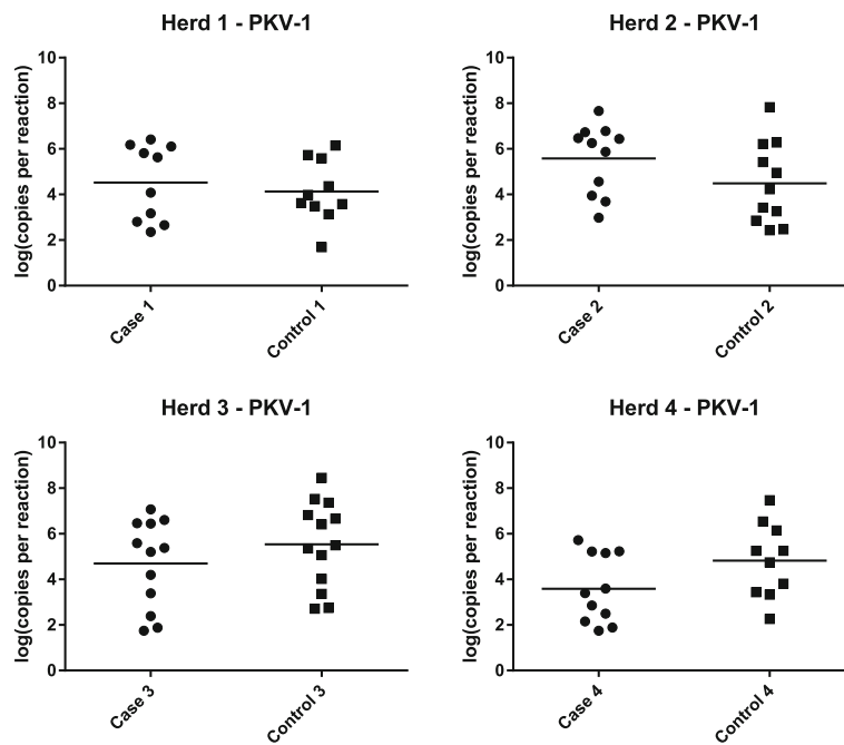
Fig. 1 Viral load (log 10 copies per reaction) of PKV-1. The copy number for the positive PKV-1 samples in herd 1–4 for case and control pigs. The straight line shows the mean value
