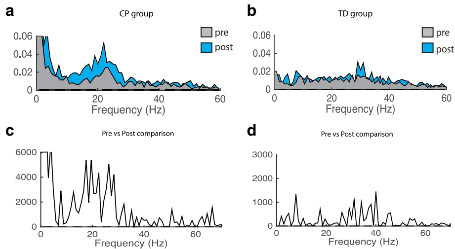
Fig. 1 Changes in FDI_LPB coherence following 3 weeks of climbing training. a-d. EMG_{APB}-EMG_{FDI} coherence. Pooled Inter-muscular coherence data from EMG_{APB}-EMG_{FDI} for the children with CP ( N = 10 , P16 included in the analysis, P7 excluded according to missing data) and TD ( N = 6 ) group respectively. Coherence is calculated from 3.5 s hold phase in 90 trials. A and B shows pooled coherence pre (light gray) and post (light blue) climbing. c and d show the \chi^2 extended test for differences of coherence. Note that the \chi^2 values give the statistical differences between the measurements and that peak values of \chi^2 values may indicate both an increase and decrease in coherence. It is therefore not possible to determine from the bottom line of graphs which of the measurements was the largest. This can only be determined from the above graph. The dashed horizontal lines in all plots denote the 95% confidence limits \chi^2
