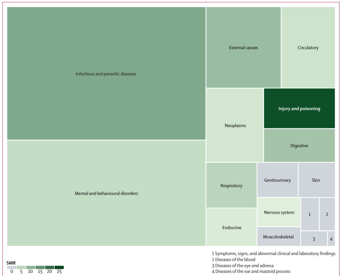
Figure 2: Treemap summarising the amount of available data grouped according to the ICD-10 disease categories and summary estimates of SMRs. Box sizes indicate the total number of datapoints included in this Article. SMRs used are summary estimates for the ICD-10 disease categories for both sexes combined. Grey boxes (SMR of 0) indicate that none of the studies included in this Article reported SMR for both sexes combined. ICD-10=International Classification of Diseases, tenth revision. SMR=standardised mortality ratio.
