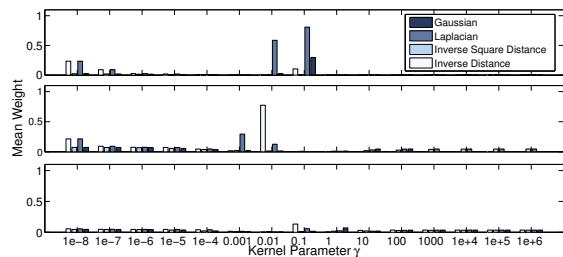
(a) K_{CKA}
