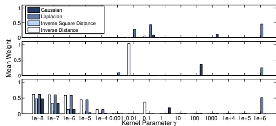
(c) K_{W_{MMD}}
