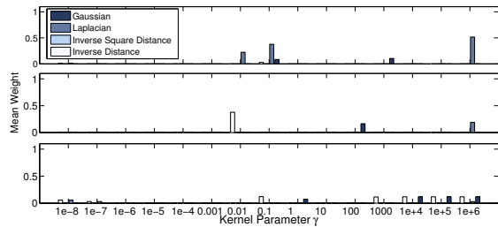
(b) K_{MMD}
